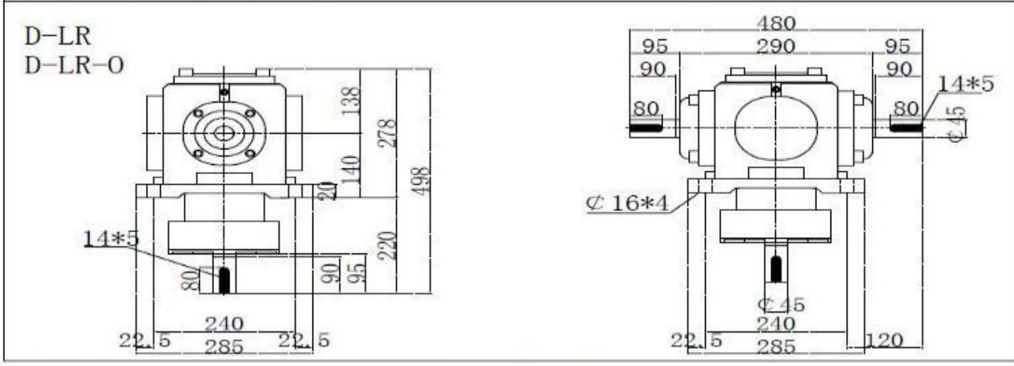
SJ-T12 Bevel Gearbox Dimensions
