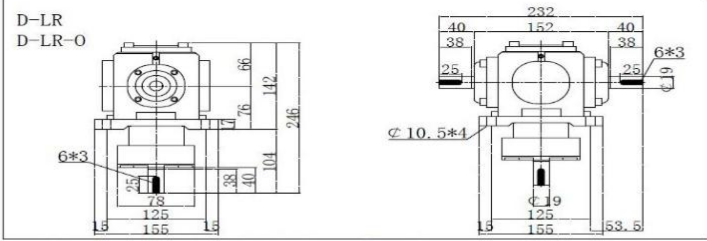
SJ-T6 Bevel Gearbox Dimensions
