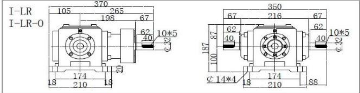
SJ-T7 Bevel Gearbox Dimensions
