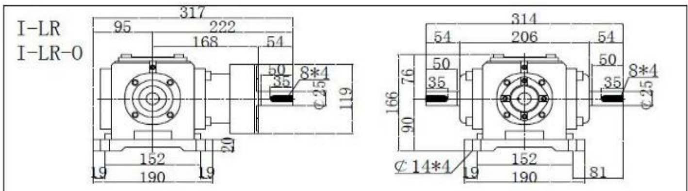
SJ-T6 Bevel Gearbox Dimensions
