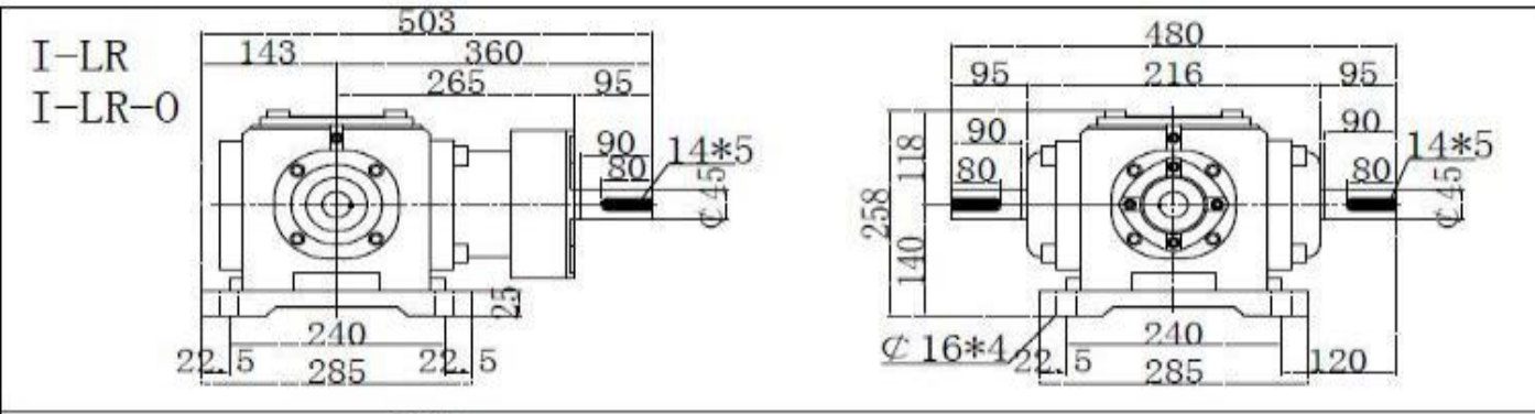
SJ-T10 Bevel Gearbox Dimensions
