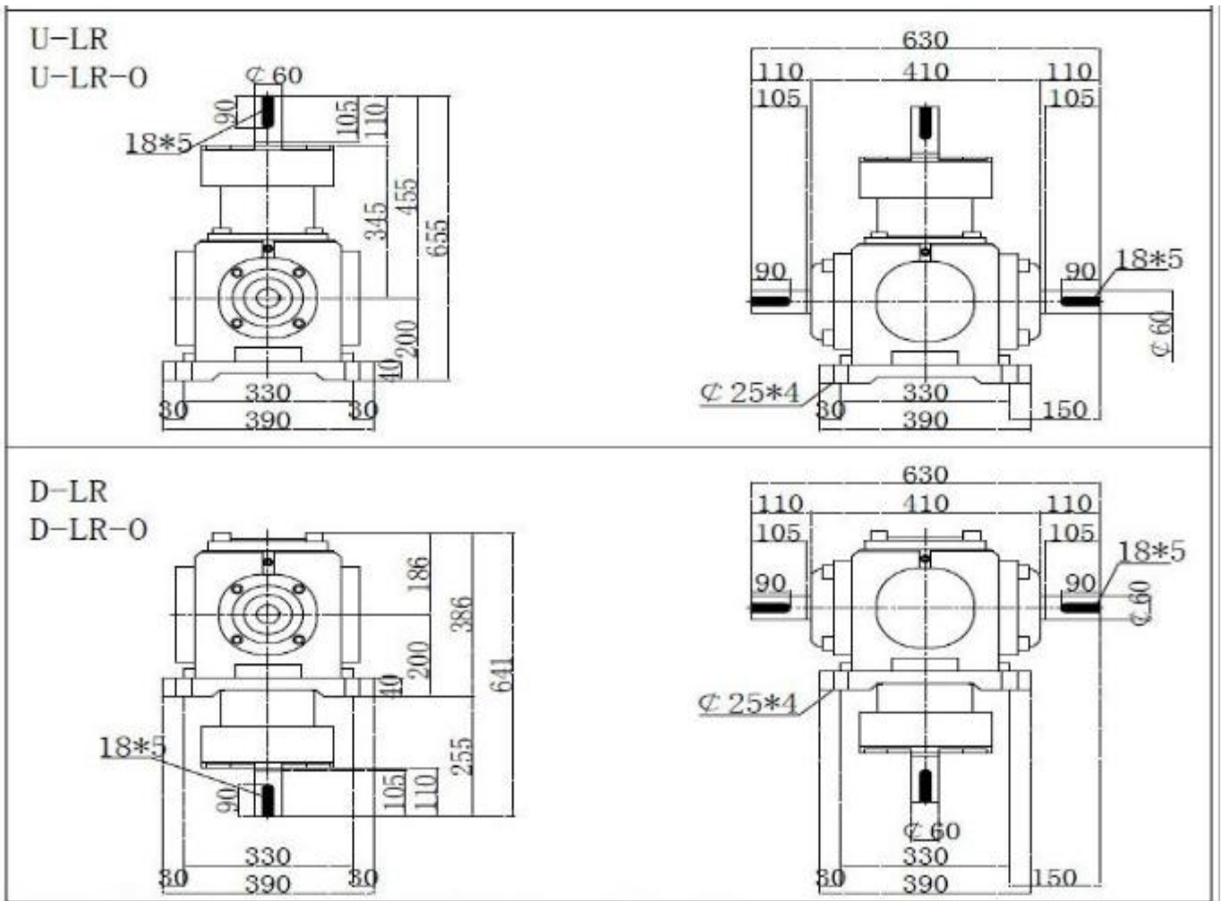
SJ-T20 Bevel Gearbox Dimensions
