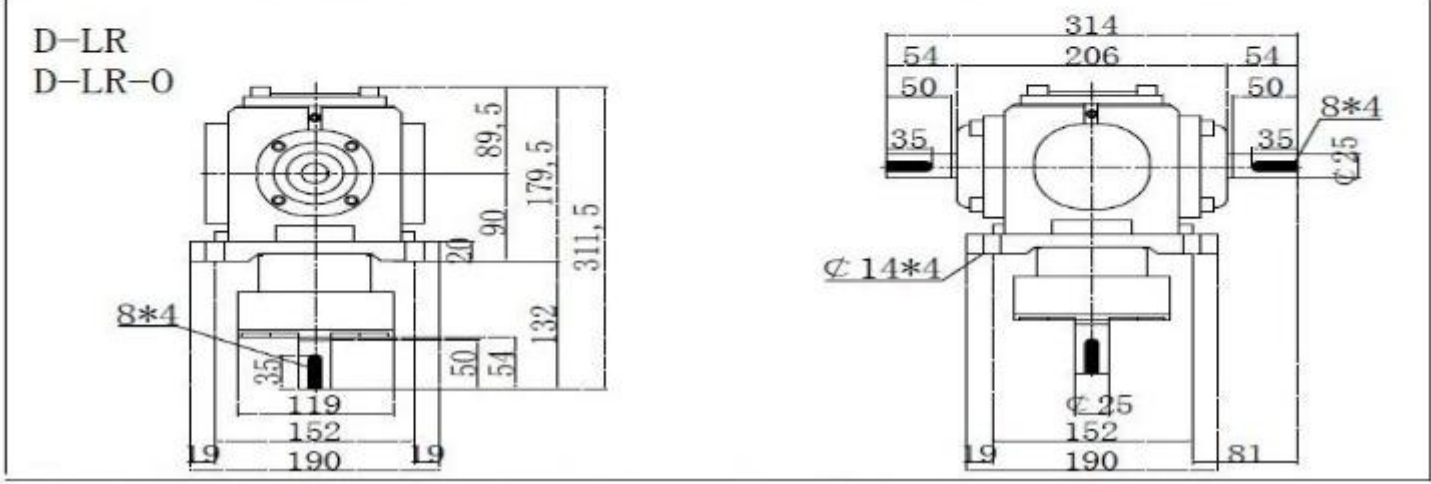
SJ-T7 Bevel Gearbox Dimensions
