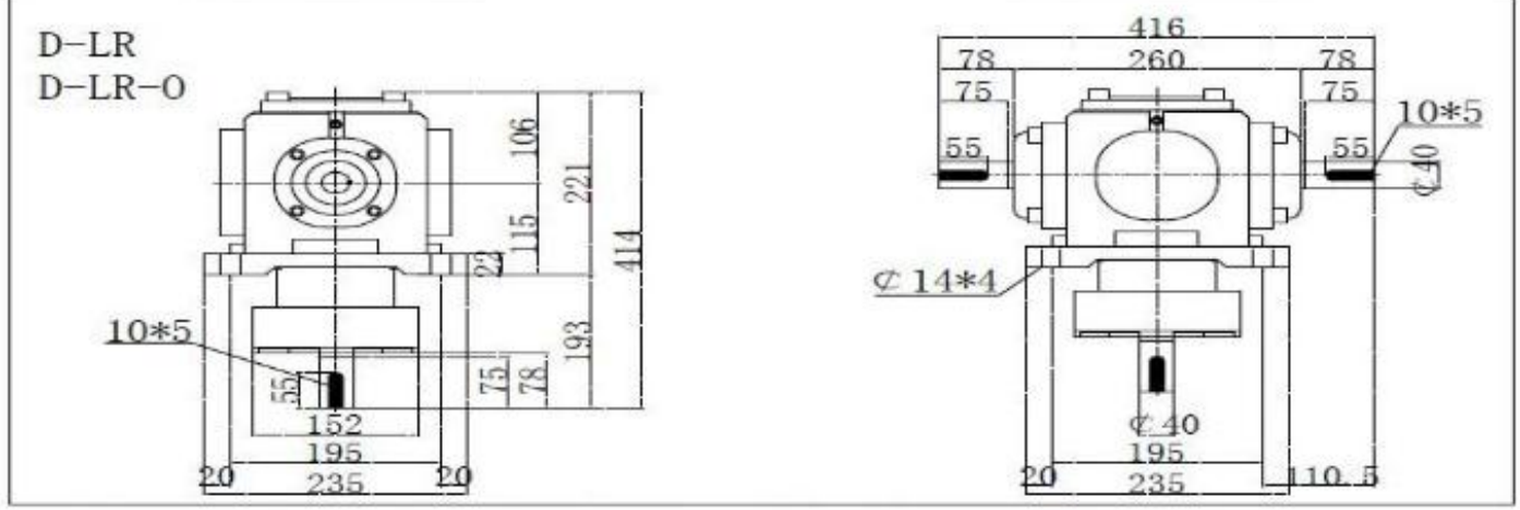
SJ-T10 Bevel Gearbox Dimensions
