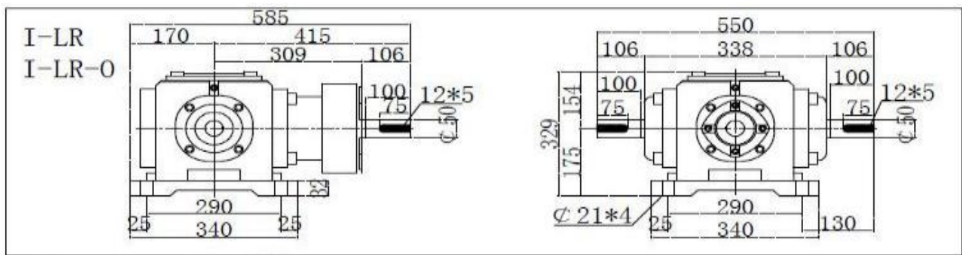
SJ-T12 Bevel Gearbox Dimensions
