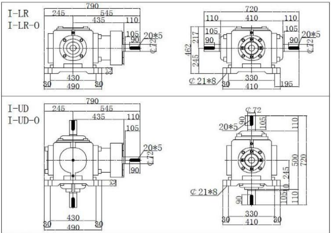
SJ-T20 Bevel Gearbox Dimensions
